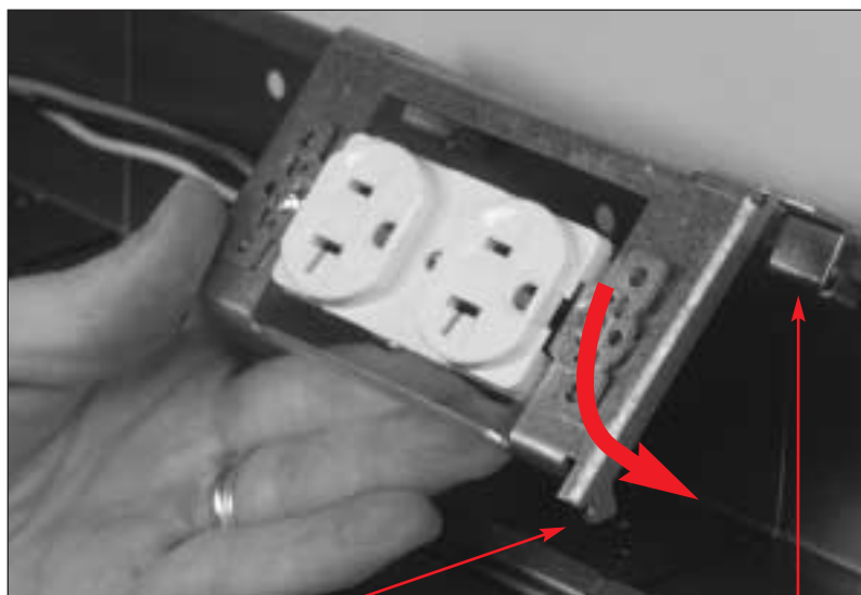
Rotate Bracket down and snap into place.
