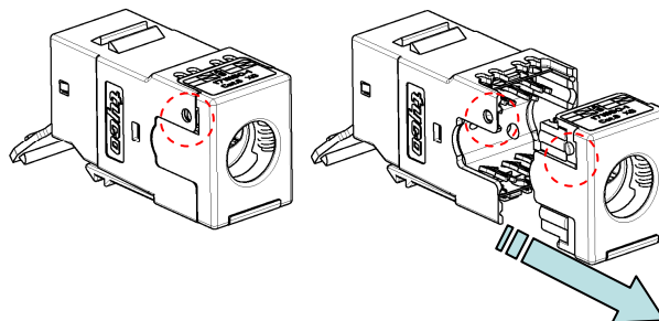
Figure 8 Front/Rear Housing retention
