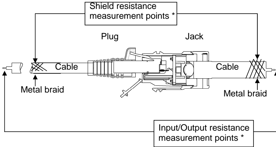
Figure 6 Input/Output and shield resistance measurement points as shown
