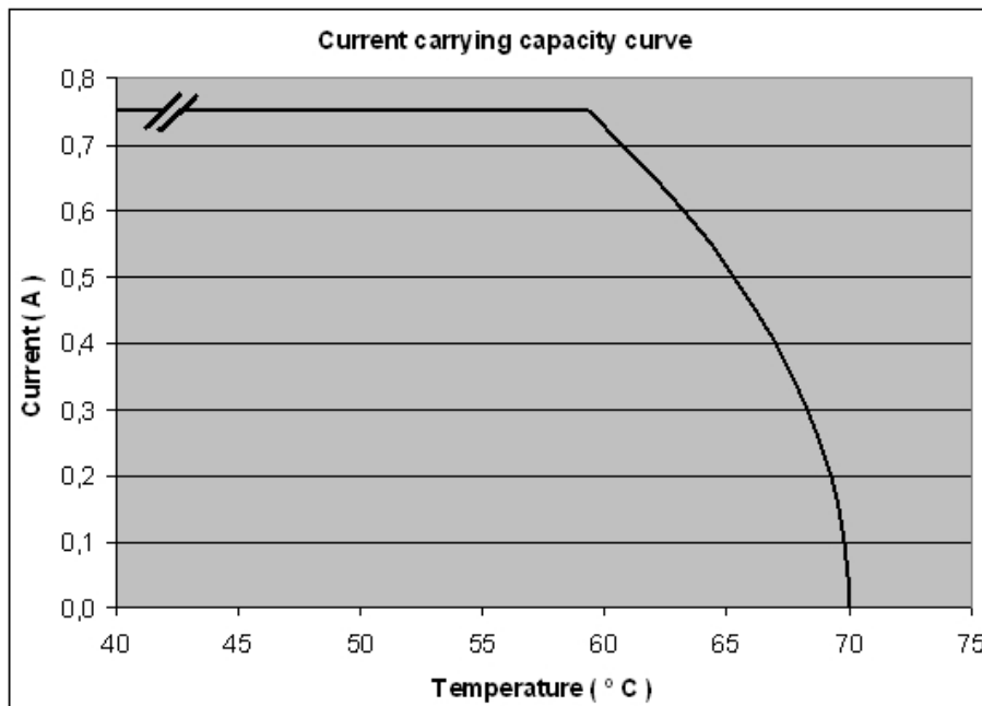
Figure 5 Current-carrying capacity
