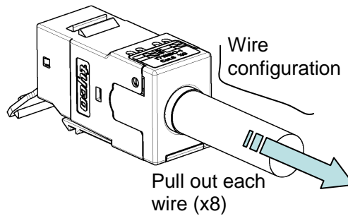
Figure 7 Termination Tensile Strength Vertical Pull
