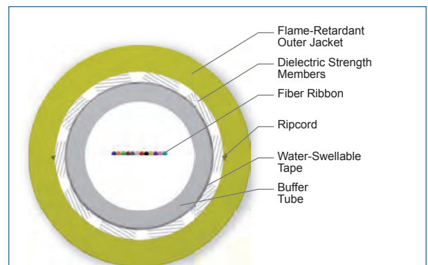
Cross Section of Part Number: 012EC8-14101-20
