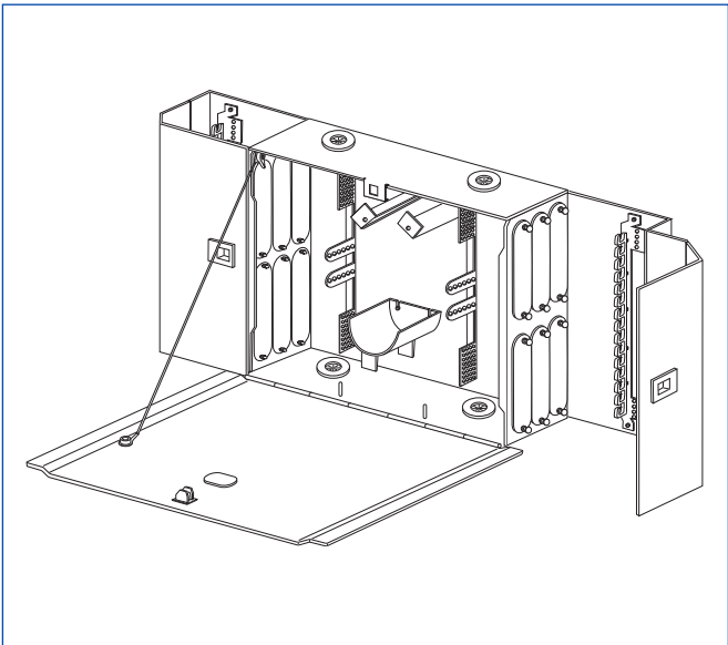
WCH-12P (up to 144 fibers) | Drawing CPC-220/5/31
