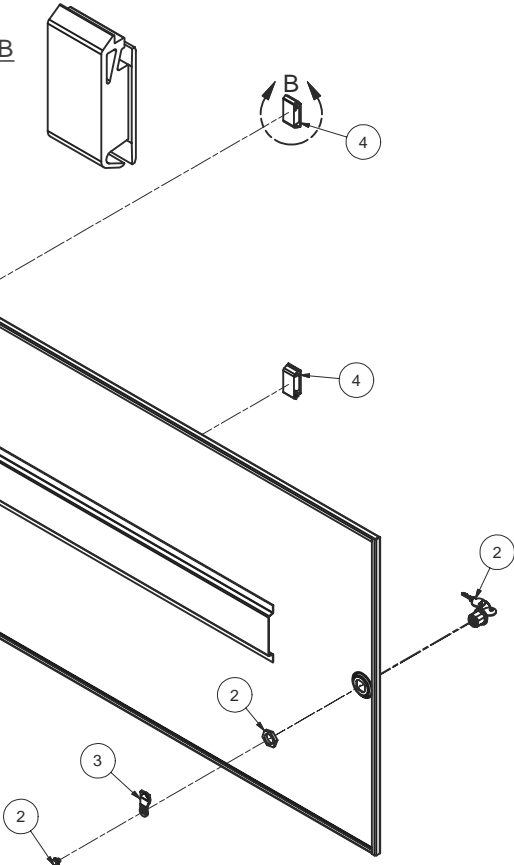
EXPLODED VIEW OF LOCK AND CAM CAM SHOWN IN UNLOCKED POSITION
