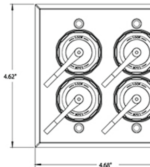
Industrial Outlet Kit, Dual-Gang, QuickPort connectors sold separately.
