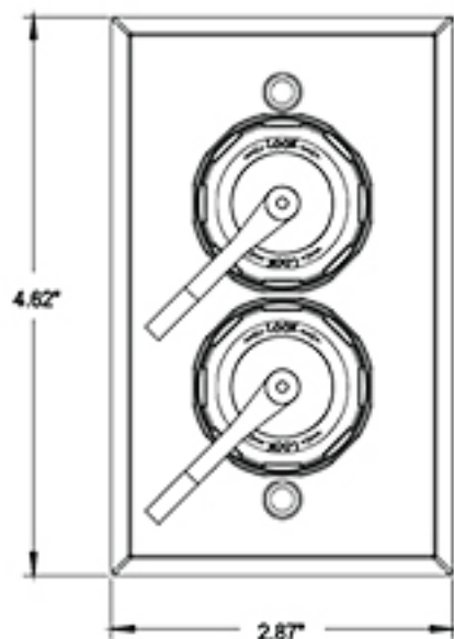
Industrial Outlet Kit, Single-Gang, 2-Port QuickPort Connectors sold separately.
