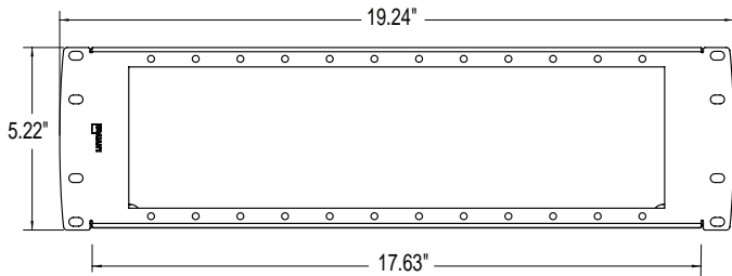
5R3UL-F12
