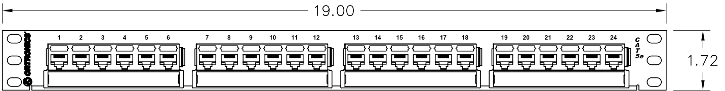
FRONT VIEW
